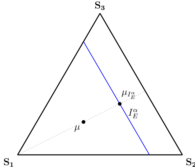
Figure 3: \alpha -event and Bayesian Updating for E = \{s_2, s_3\} and \alpha = 0.8 .
