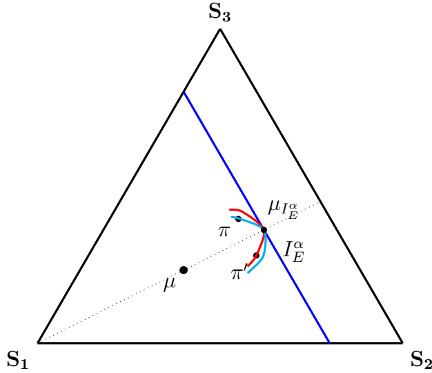
Figure 4: \alpha -event and Bayesian Updating for E = \{s_2, s_3\} and \alpha = 0.8 .
