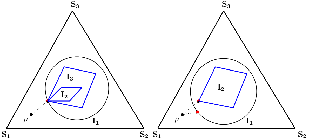
Figure 2: Illustrations of Informational Betweenness (left) and Extremeness (right).
