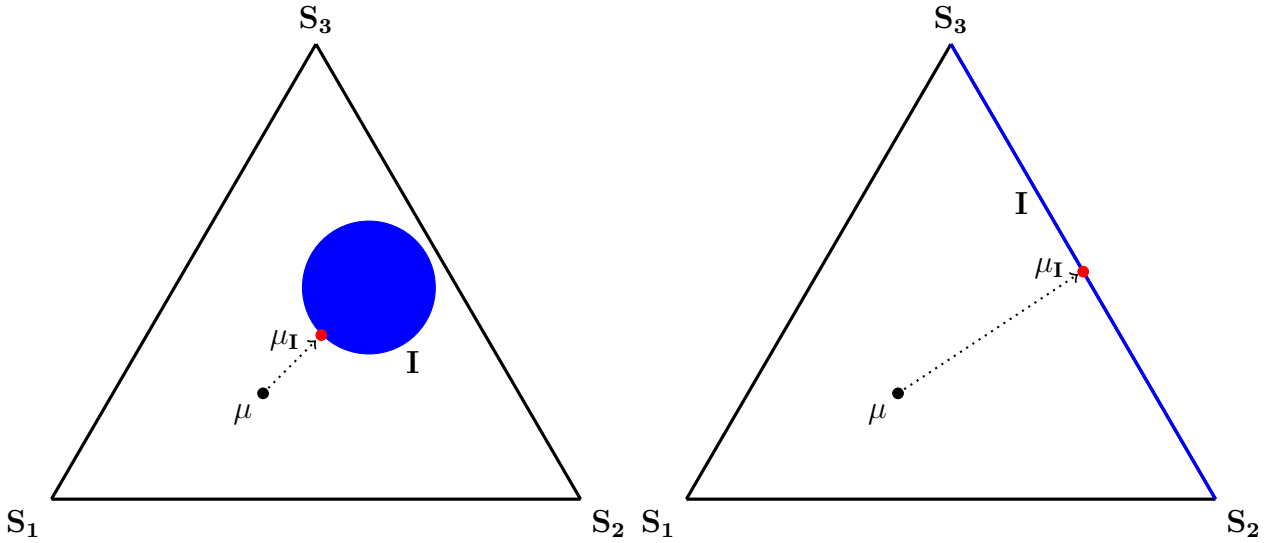
Figure 1: Information Sets and Minimum Distance Updating.
